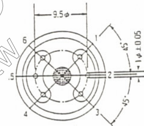
Dimensions in millimeter
